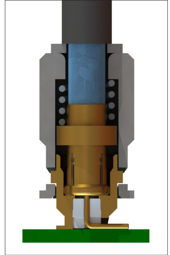
Figure 2: A cross-section of a mated QB pair showing the spring loaded action that makes this product line quick to mate.
