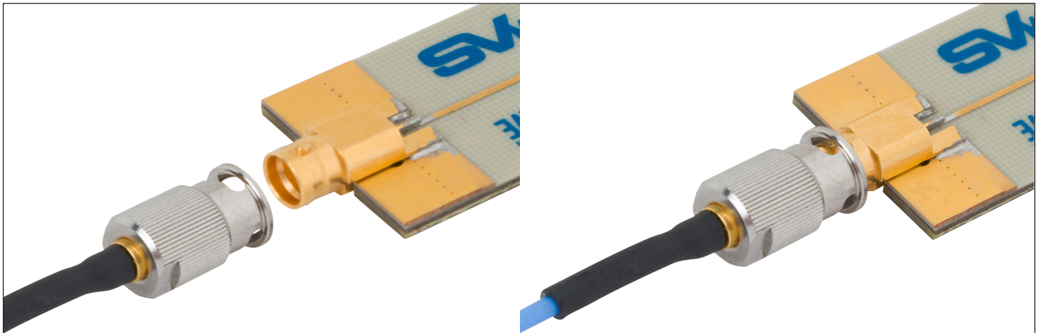
Figure 1: An SMP Female QB Cable Assembly (7012-1300) is shown with an SMP Male PCB QB Edge Launch Connector, SB in both the unmated and mated positions.
