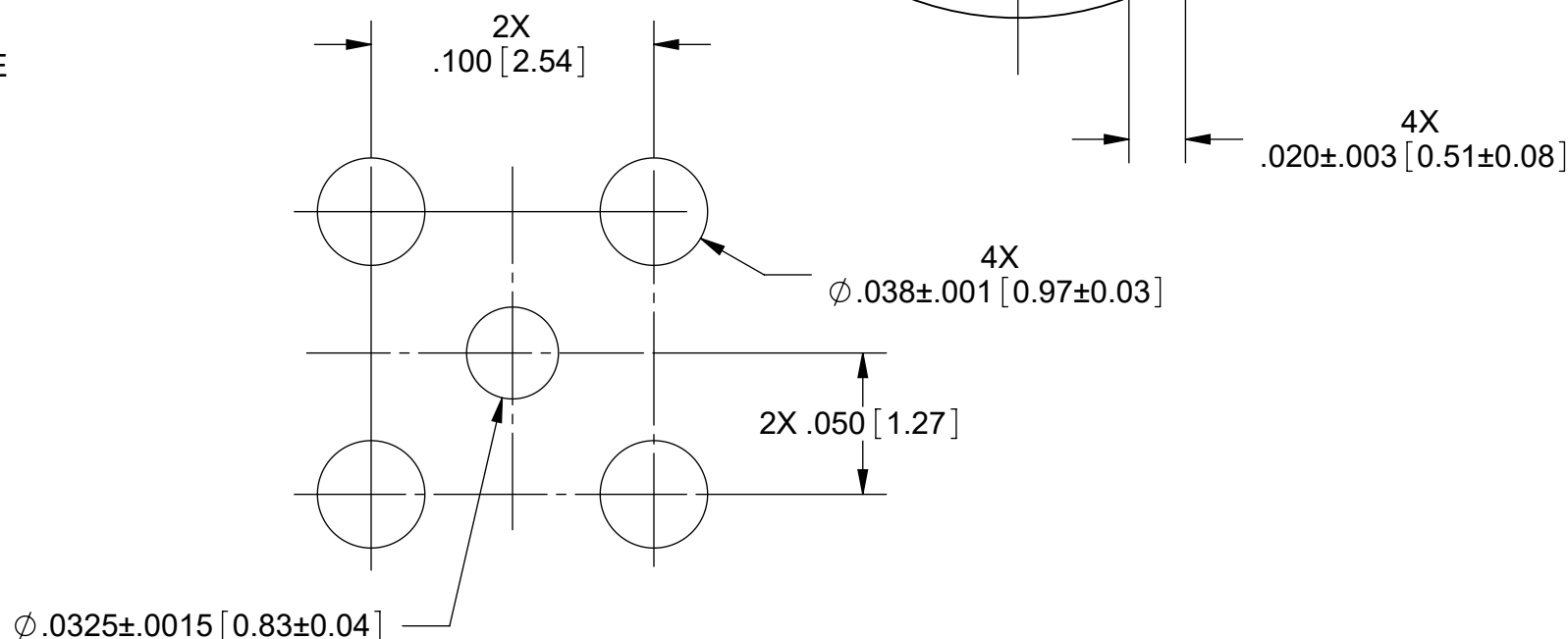
RECOMMENDED MOUNTING HOLE PATTERN
