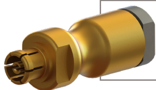
3221-40128* SMPM Straight Female for SuperFlex Ø.047
